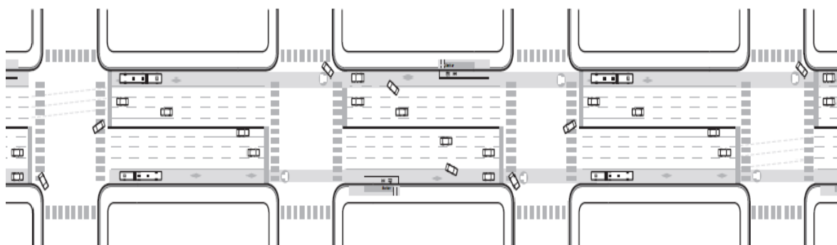
Figure 1 Kerbside BRT concept – typical lane configuration Source VTA Transit Sustainability Policy, 2007
