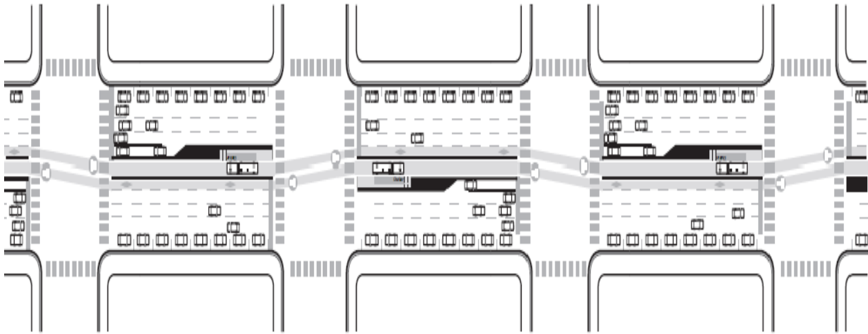
Figure 2: Median BRT system – typical lane configuration
