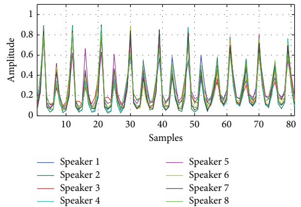
FIGURE 24: Time domain plot of the LPCC-HOG features for the utterance “Hello Hello Hello . . .” of the first 8 Speakers.
