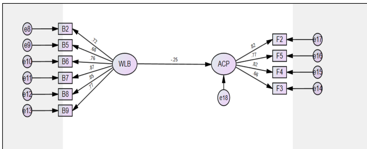
Figure 1: Measurement Model (authors own)
