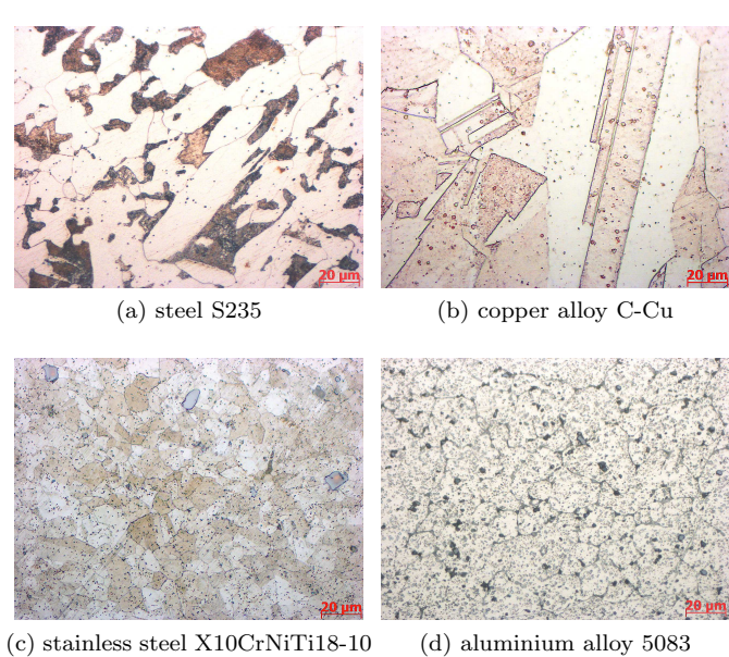
FIG. 1: Microstructure of the studied materials.
