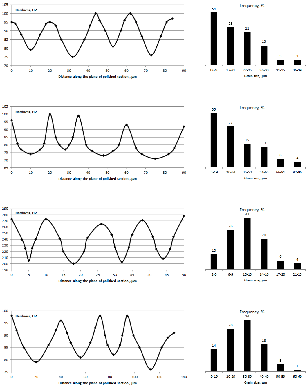
FIG. 2: Hardness profiles (left column) and grain size distributions (right column) in, from top to bottom: ferrite S235, copper alloy C-Cu, austenite X10CrNiTi18-10, and aluminium alloy 5083.
