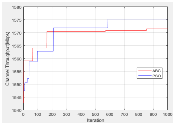
Fig. 9: Sum throughput when SUs = 200, Channels = 30
