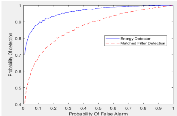
Fig. 6: False alarm probability Vs detection probability
