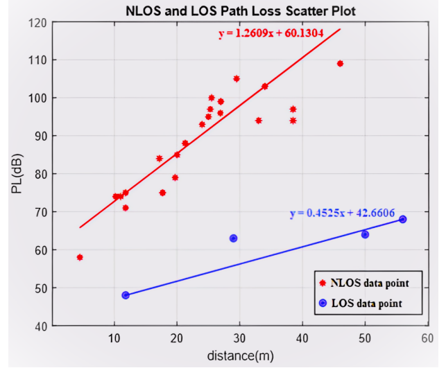
Fig. 13. Log-normal shadowing regression line model for NLOS and LOS.
