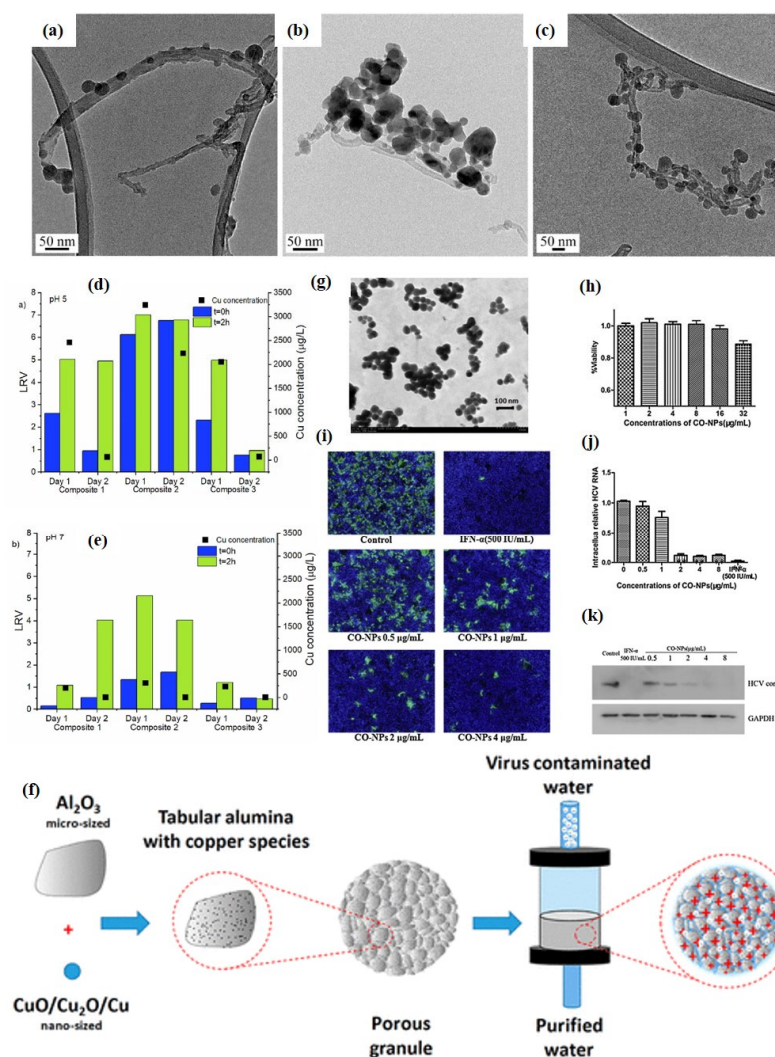
Figure 15. TEM images of Cu 2 O-MWCNTs nanocomposites: (a) composite 1; (b) composite 2; (c) composite 3. MS2 removal test results for composite 1, composite 2 and composite 3 at (d) pH 5 and (e) pH 7, and the associated copper concentrations detected in the permeate (reproduced with permission from Ref. [114] Copyright 2020-Elsevier); (f) Schematic representation of nano-sized copper (Oxide) on alumina granules filters for water filtration. Reproduced with permission from Ref. [115] Copyright 2020, American Chemical Society. Cu 2 O (CO) NPs inhibited HCV infection. HCVcc (MOI = 0.1) virions were added with the indicated concentrations of Cu 2 O NPs or interferon- (IFN- \alpha , 500 IU/mL) to Huh7.5.1 cells. After incubation at 37 °C for 2 h, the cells were washed three times to remove the virus and treated with the indicated concentrations of Cu 2 O NPs for additional 72 h; (g) the TEM image of Cu 2 O NPs; (h) Huh7.5.1 cells were treated with Cu 2 O NPs at the indicated doses for 72 h. The effect of Cu 2 O NPs on cell viability was measured by a CCK8 assay kit; (i) Huh7.5.1 cells at 72 h post-infection were stained with HCV-positive serum from patients and with DAPI. Representative fluorescence images are shown (80 \times magnification); (j) The intracellular HCV RNA content was determined by qRT-PCR; and (k) Western blot analysis of the harvested cell lysates using the anti-core or anti-GAPDH antibodies. Results are represented as the mean \pm SD from 3 independent experiments ( p < 0.001 ) (reproduced with permission from Ref. [117]. Copyright 2015-Elsevier).
