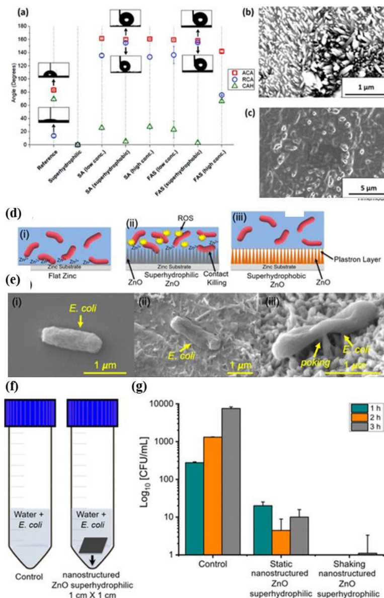
Figure 11. (a) Wetting properties using contact angle measurements done for different ZnO based samples. SEM micrographs of: (b) SA-coated; (c) FAS-coated ZnO nanostructures; (d) schematic representation mode of interactions of surface–bacteria on flat Zn substrates, nanostructured superhydrophilic ZnO surfaces, and nanostructured hydrophobized ZnO surfaces; (e) SEM micrographs of E. coli on (i) glass coverslip, (ii) flat zinc, and (iii) nanostructured ZnO superhydrophilic surface; and (f,g) ZnO superhydrophilic surfaces in inactivation of E. coli in water disinfection under static and shaking conditions. (reproduced with permission from Ref. [85] copyright-2020 American Chemical Society).
