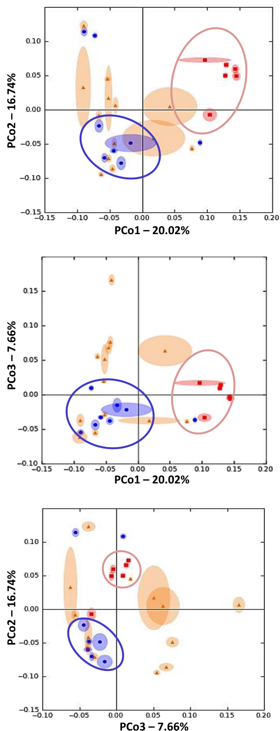
Figure 3 PCoA of unweighted UniFrac distances between samples analyzed by TTGE. Principal coordinate analysis of unweighted UniFrac distances between Ae. aegypti larvae and water from mosquito positive and negative containers. Distinct clusters of larval samples (red) and mosquito positive water samples (blue) are captured on all three PCoA plots. Mosquito negative water samples (orange) do not show any distinct clusters on any of the plots. Each axis show percentage of variation explained. Each data point consists of a central point surrounded by ellipsoids that indicate variation in UniFrac distances from rarefaction. This demonstrates that the clustering pattern holds up to subsampling.
