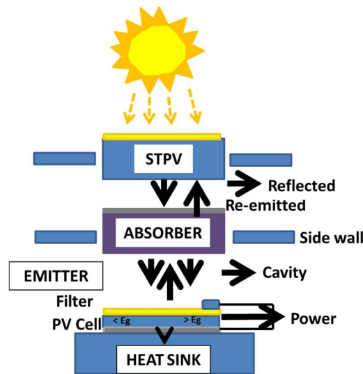
FIGURE 1. STPV and its energy flow flowchart [13].
