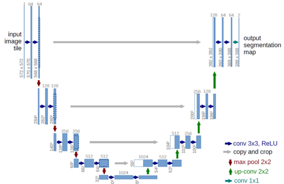
Fig. 9. Architecture of the U-Net
