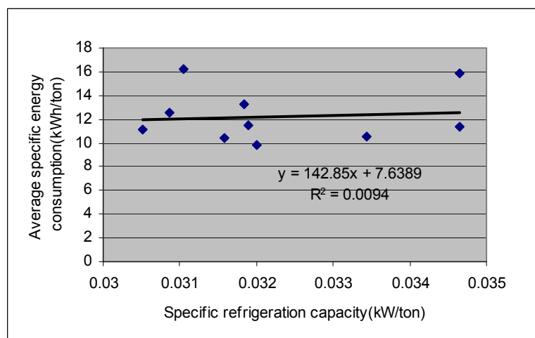
Figure 8. SEC vs. Specific refrigeration capacity
